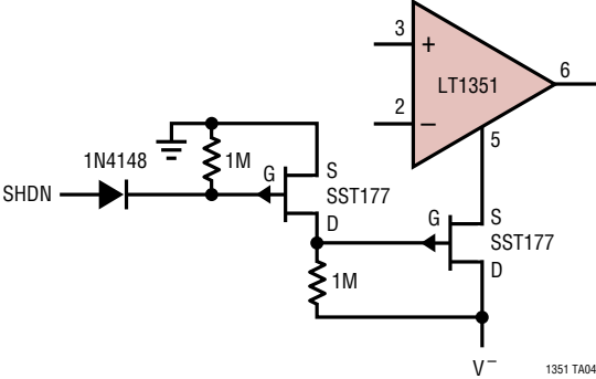
Shutdown Circuit
